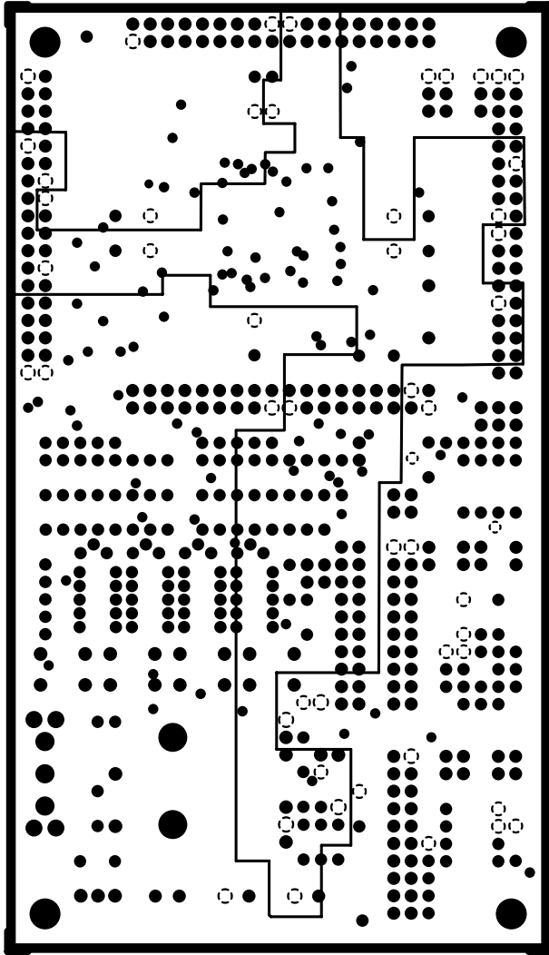
V33 VCCINT Internal Plane 2
