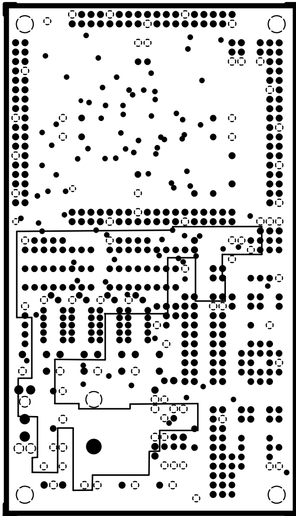
GND V50 Internal Plane 1
