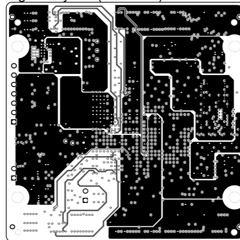
Signal Layer 6 (Scale 1:1)
