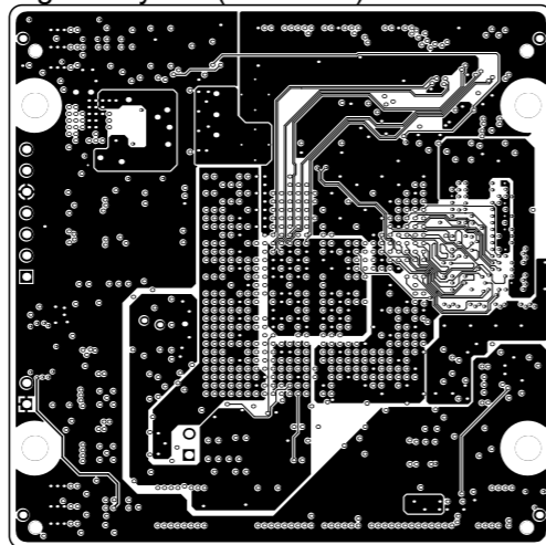
Signal Layer 2 (Scale 1:1)
