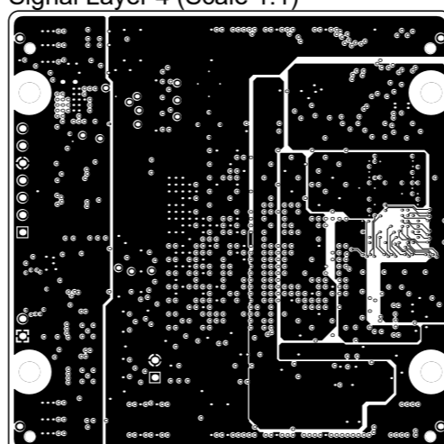
Signal Layer 4 (Scale 1:1)
