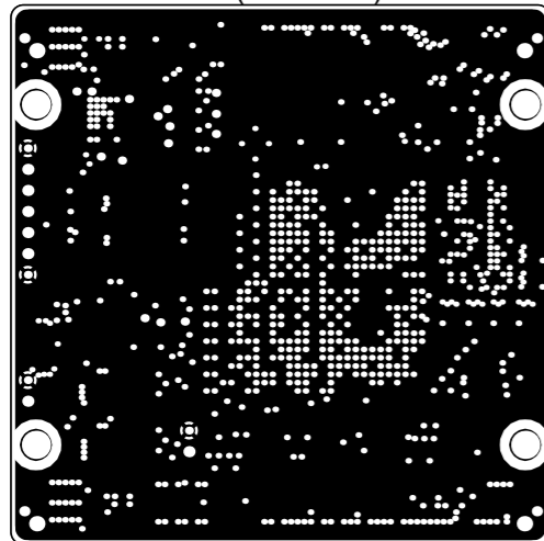
Internal Plane 1 (Scale 1:1)
