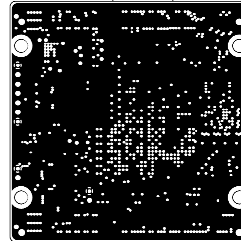
Internal Plane 2 (Scale 1:1)
