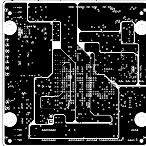
Signal Layer 3 (Scale 1:1)
