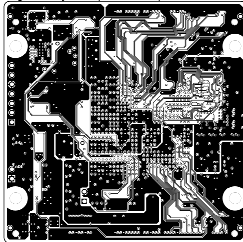
Signal Layer 1 (Scale 1:1)
