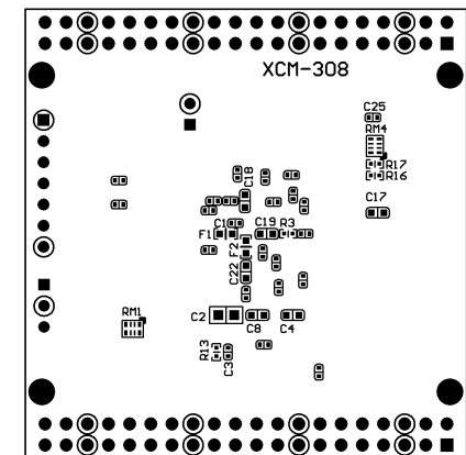
Solder Side
