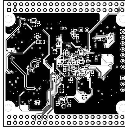
BottomLayer (Scale 1:1)
