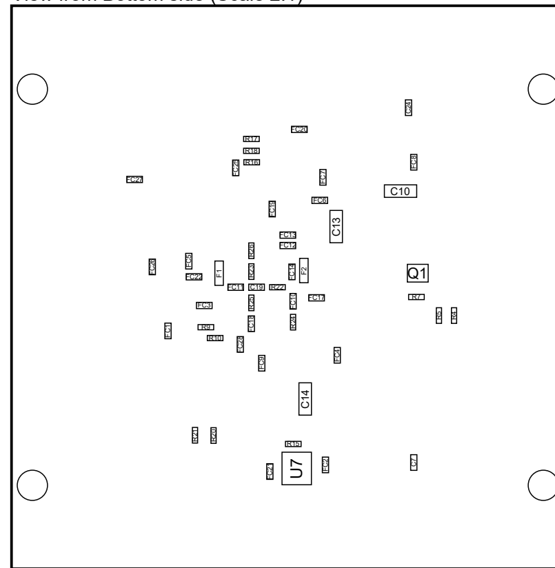
View from Bottom side (Scale 2:1)
