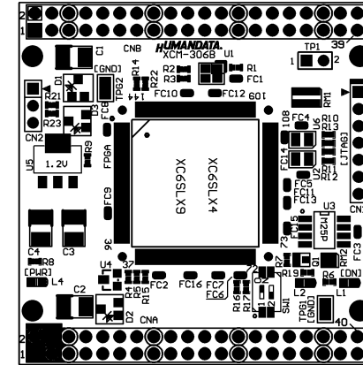
Component Side
