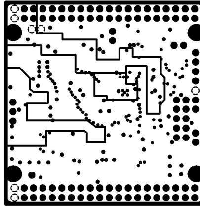
INTERNAL PLANE2(VCC)
