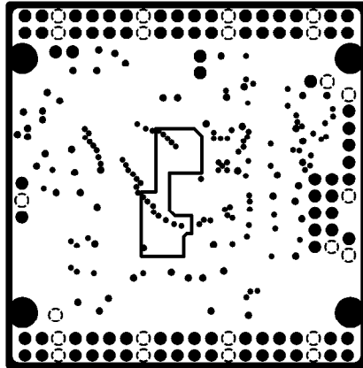
INTERNAL PLANE1(GND)
