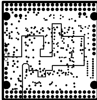
INTERNAL PLANE3
