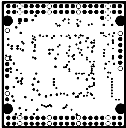
INTERNAL PLANE1(GND)
