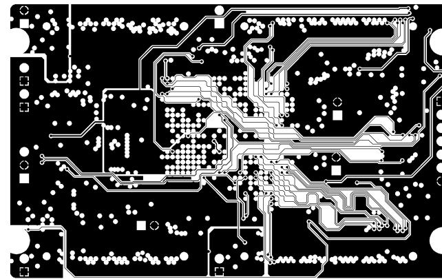
SIGNAL LAYER 2
