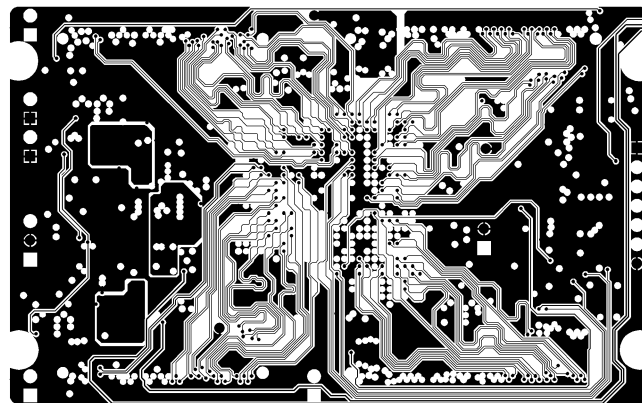
SIGNAL LAYER 1
