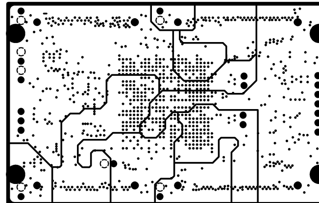
INTERNAL PLANE 4
