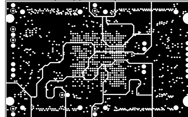
Power Plane (VCC) (Scale 1:1)
