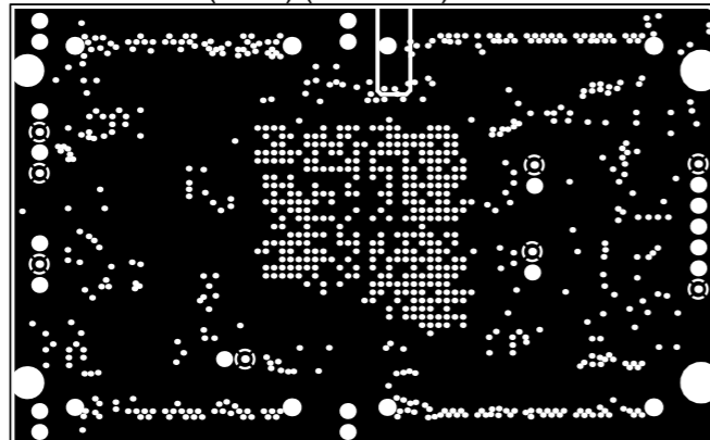
Ground Plane (GND) (Scale 1:1)
