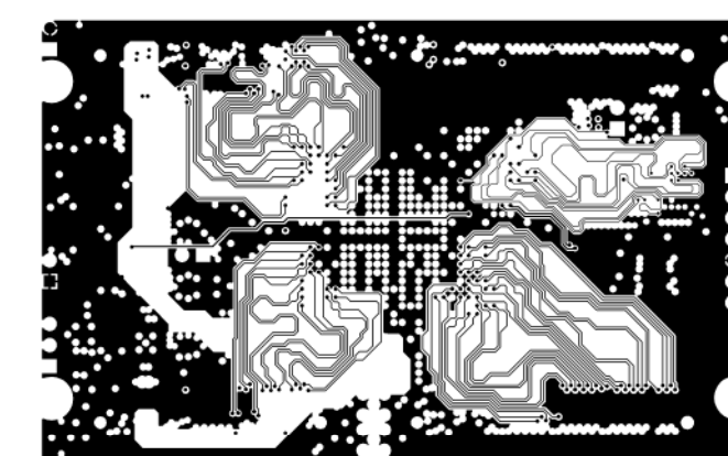
SIGNAL LAYER 3
