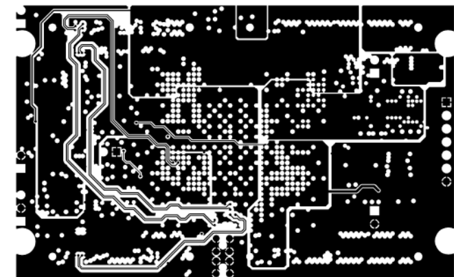
SIGNAL LAYER 4
