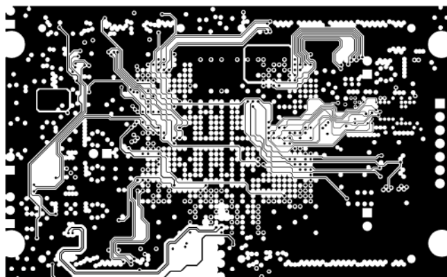
SIGNAL LAYER 2
