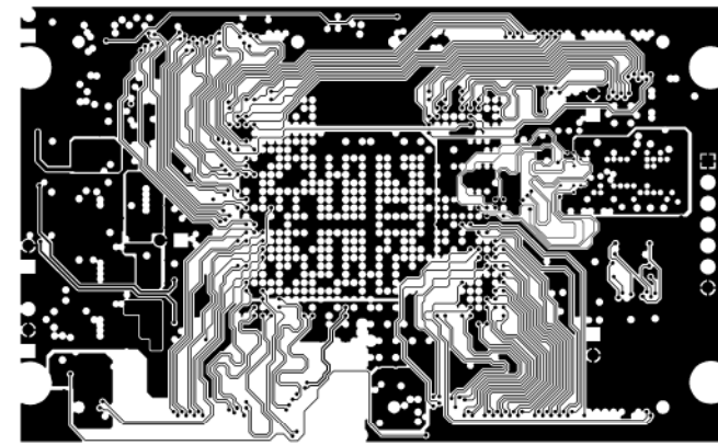
SIGNAL LAYER 1
