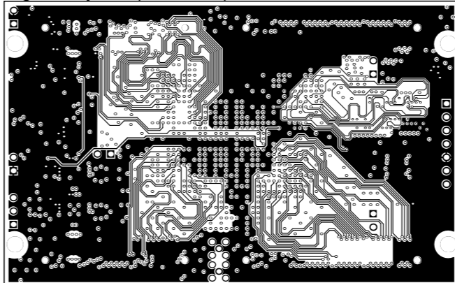
Signal Layer 3 (Scale 1:1)
