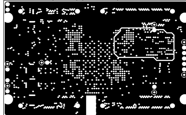
Power Plane (GND2) (Scale 1:1)
