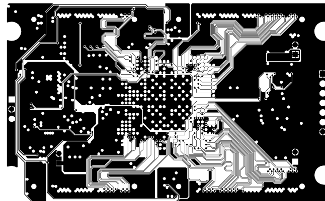
SIGNAL LAYER 1
