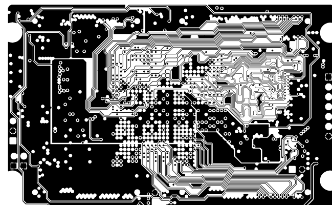
SIGNAL LAYER 2
