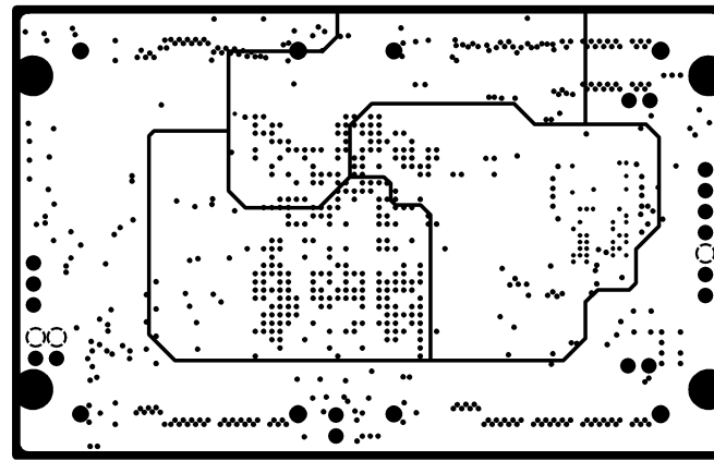
INTERNAL PLANE 4
