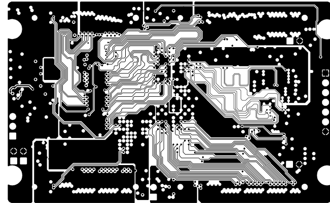
SIGNAL LAYER 3
