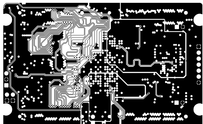
SIGNAL LAYER 4
