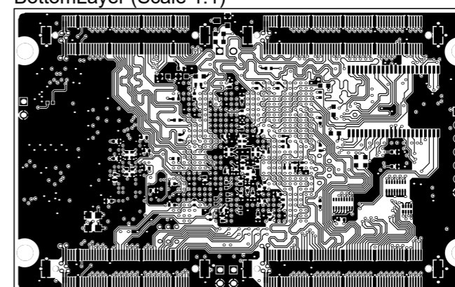
BottomLayer (Scale 1:1)
