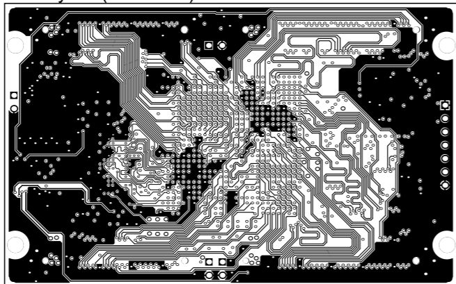
MidLayer2 (Scale 1:1)
