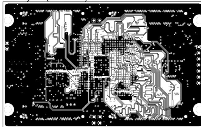
MidLayer4 (Scale 1:1)
