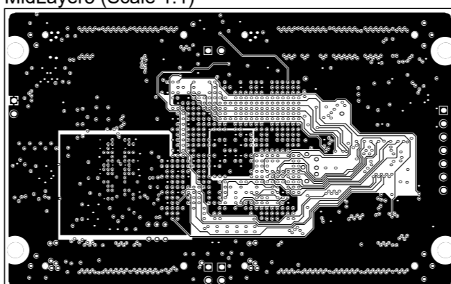
MidLayer5 (Scale 1:1)
