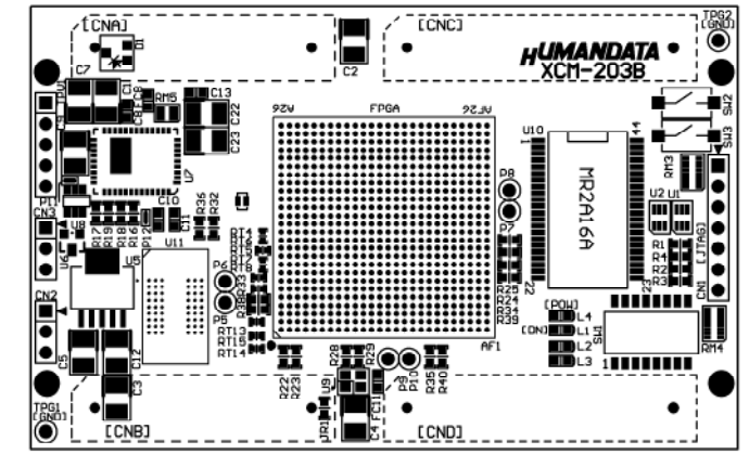
Component Side
