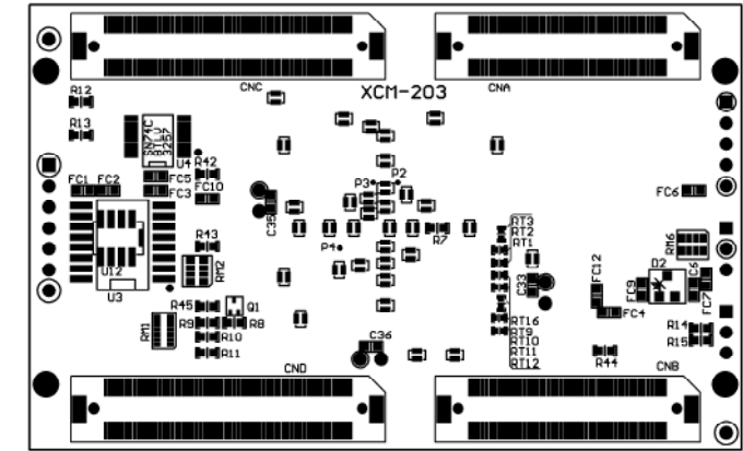
Solder Side
