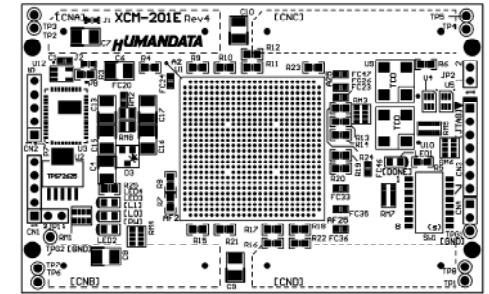
Solder Side
