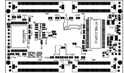
Solder Side
