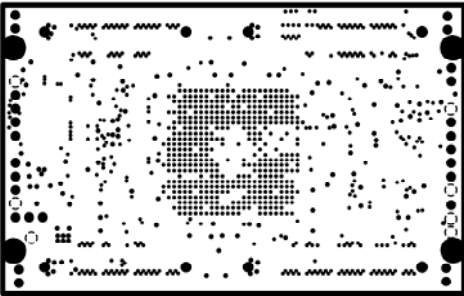
INTERNAL PLANE 1
