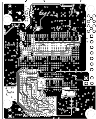
MidLayer2 (Scale 1:1)
