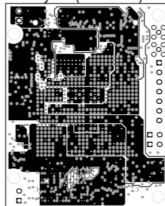
MidLayer4 (Scale 1:1)
