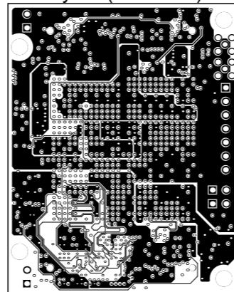
MidLayer3 (Scale 1:1)
