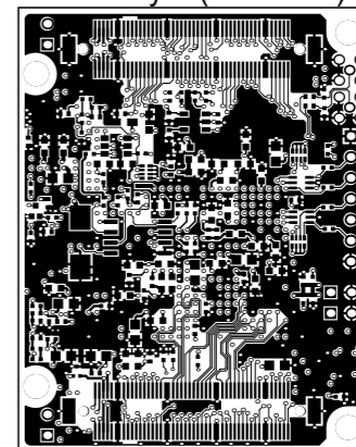
BottomLayer (Scale 1:1)
