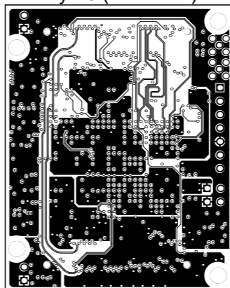
MidLayer6 (Scale 1:1)
