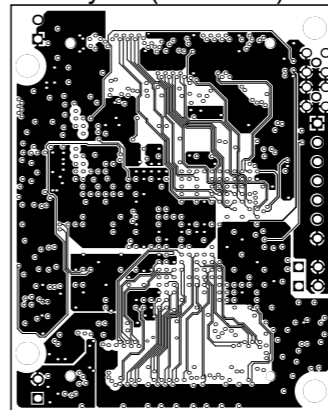
MidLayer5 (Scale 1:1)
