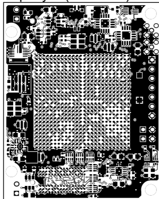
TopLayer (Scale 1:1)
