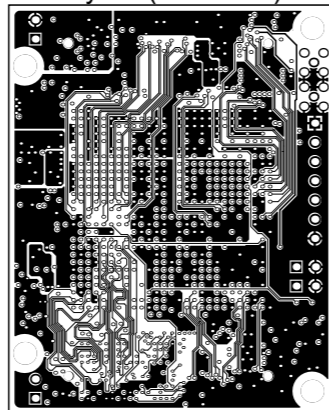
MidLayer1 (Scale 1:1)
