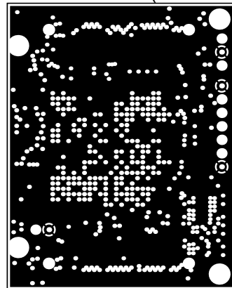
Internal Plane 1 (Scale 1:1)
