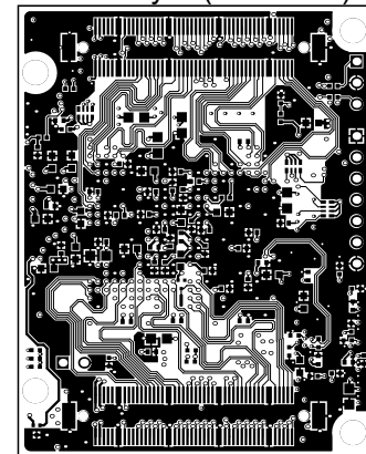
BottomLayer (Scale 1:1)
