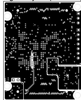
Signal Layer 4 (Scale 1:1)
