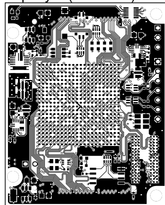
TopLayer (Scale 1:1)
