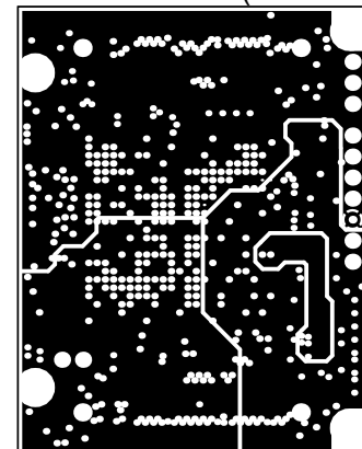
Internal Plane 2 (Scale 1:1)
