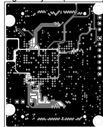
Signal Layer 3 (Scale 1:1)
