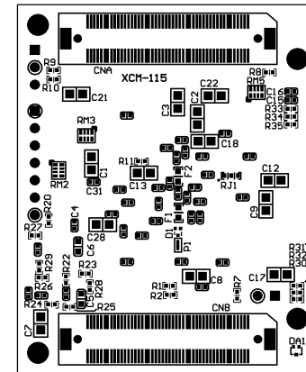
Solder Side
