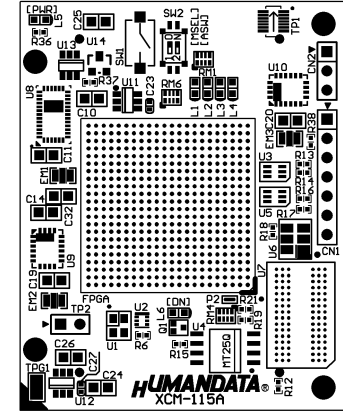
Component Side
