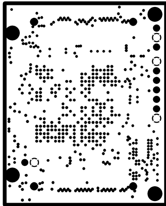
INTERNAL PLANE 1
