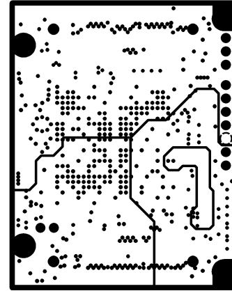
INTERNAL PLANE 2
