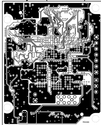
MidLayer2 (Scale 1:1)
