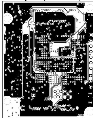
MidLayer4 (Scale 1:1)
