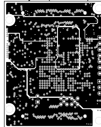
MidLayer6 (Scale 1:1)
