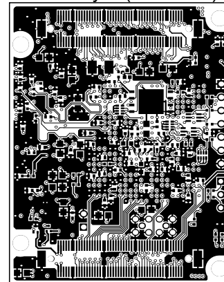
BottomLayer (Scale 1:1)
