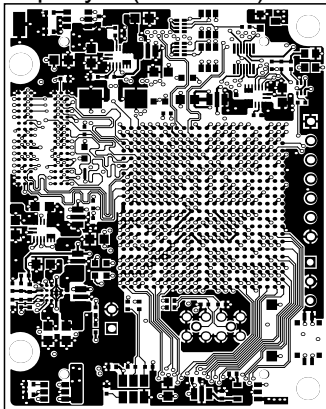
TopLayer (Scale 1:1)
