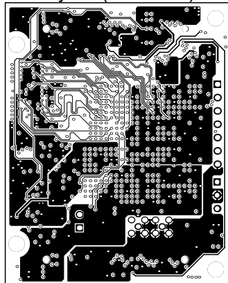
MidLayer3 (Scale 1:1)
