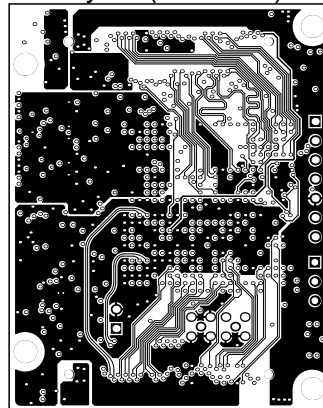
MidLayer5 (Scale 1:1)
