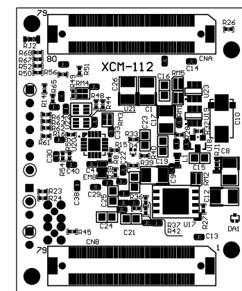
Solder Side
