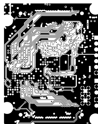
MID LAYER3
