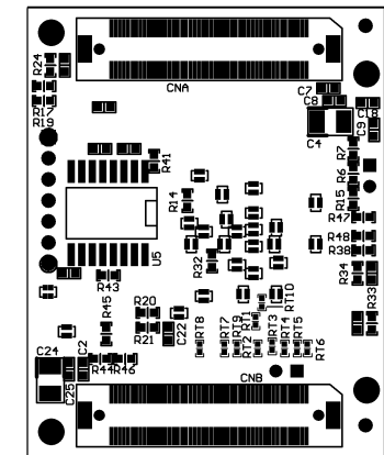
Solder Side
