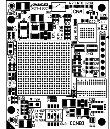
Component Side
