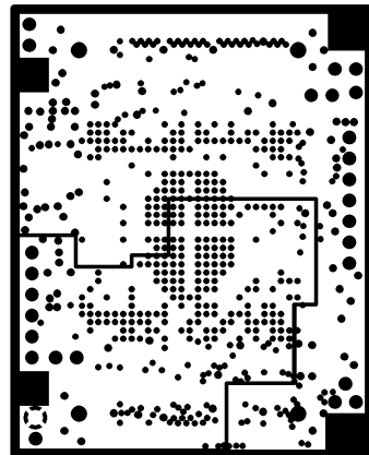
INTERNAL PLANE2(VCC)
