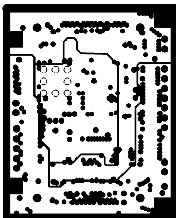
INTERNAL PLANE2(VCC)
