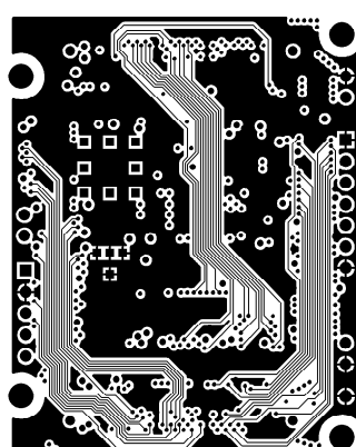
INTERNAL PLANE2(VCC)
