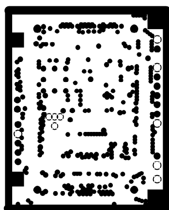
INTERNAL PLANE1(GND)
