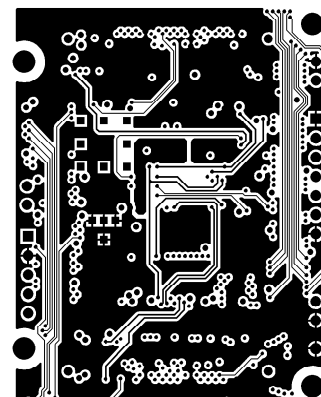
MID LAYER4
