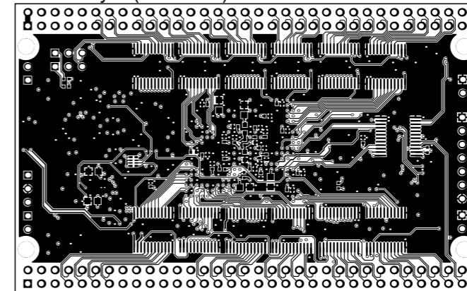
BottomLayer (Scale 1:1)
