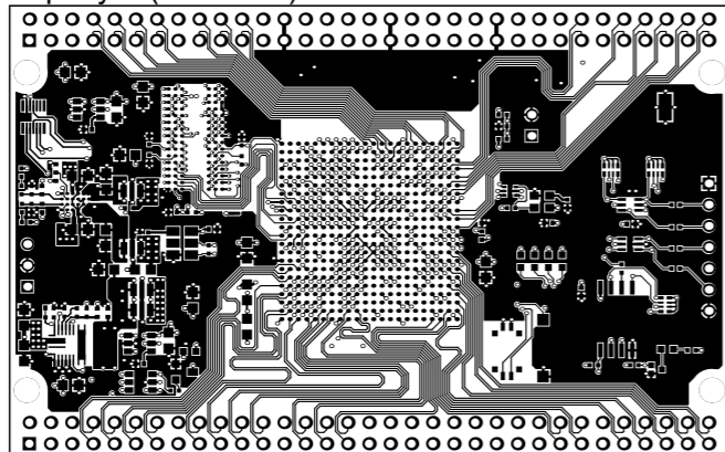
TopLayer (Scale 1:1)
