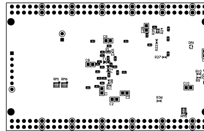
Solder Side
