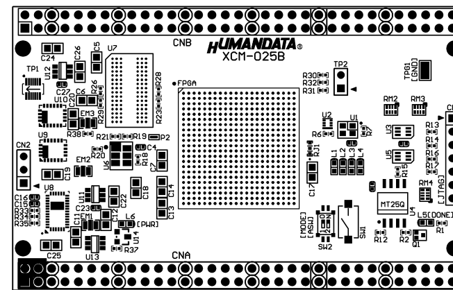
Component Side
