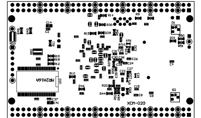
Solder Side
