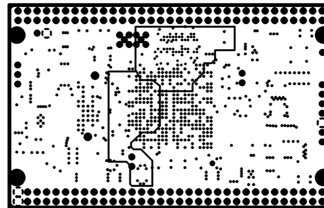
INTERNAL PLANE2(VCC)
