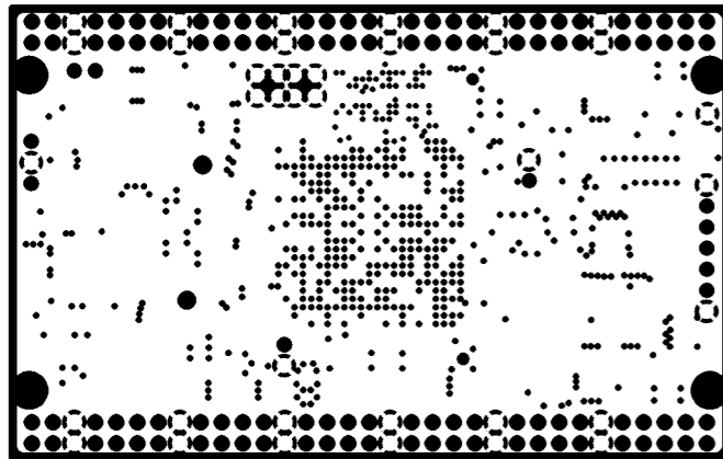
INTERNAL PLANE1(GND)
