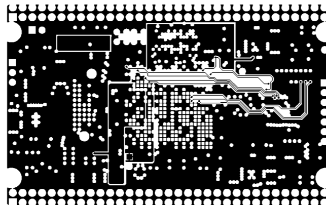
MID LAYER4
