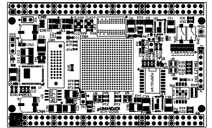
Component Side
