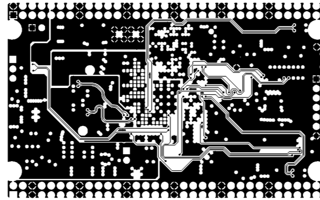
MID LAYER3
