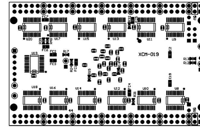
Solder Side
