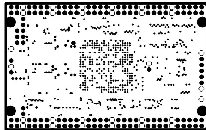
INTERNAL PLANE1(GND)
