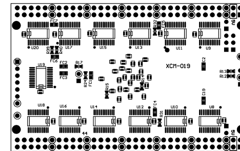
Solder Side
