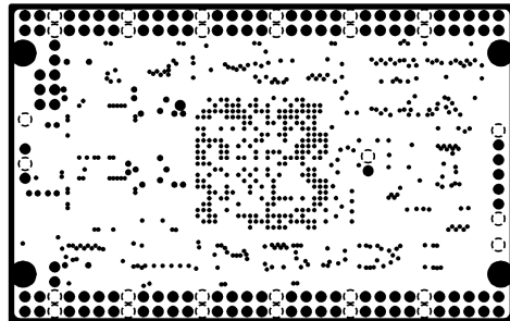
INTERNAL PLANE1(GND)
