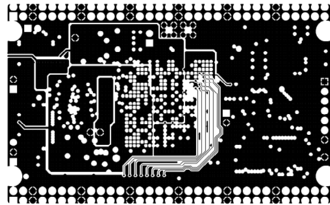
MID LAYER3
