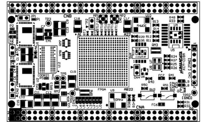
Component Side
