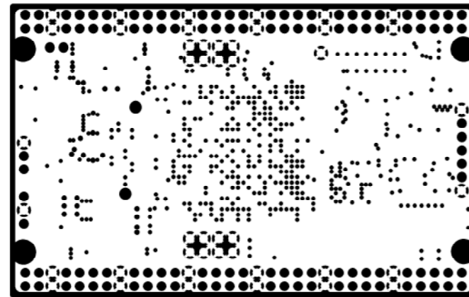
INTERNAL PLANE1(GND)
