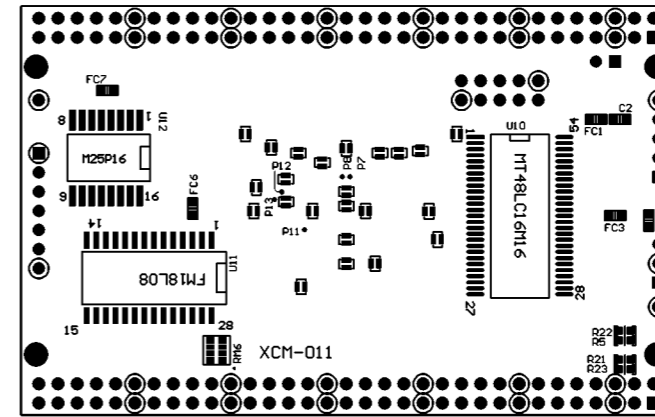
Solder Side
