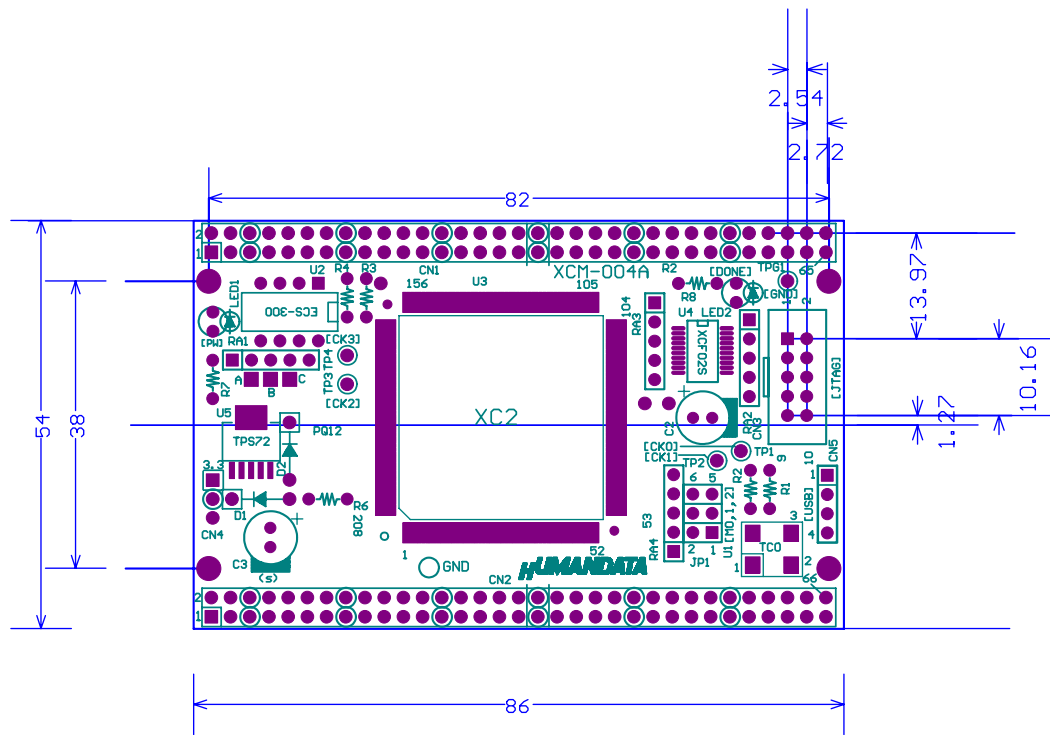
Top Solder Mask
