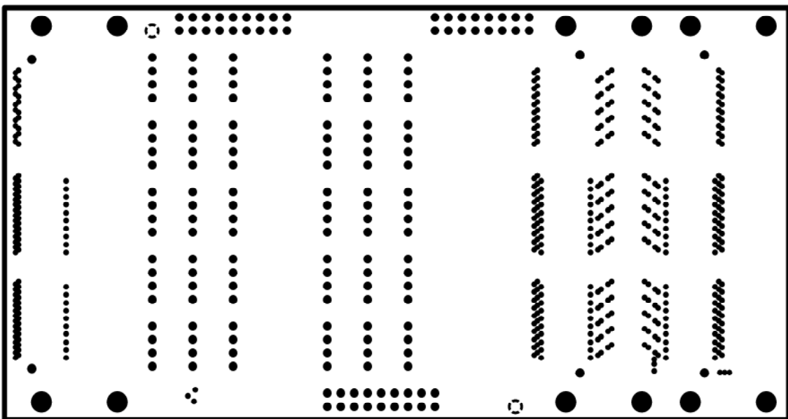
INTERNAL PLANE1
