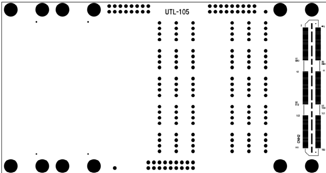
Solder Side
