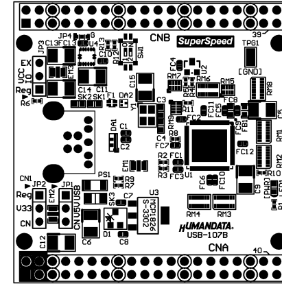
Component Side
