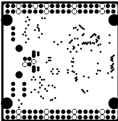
INTERNAL PLANE1
