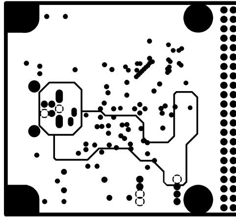
INTERNAL PLANE2
