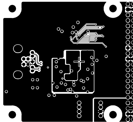
INTERNAL PLANE2
