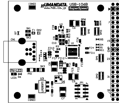
Component Side
