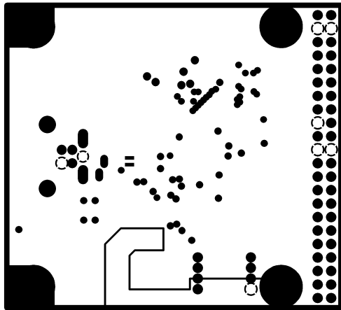
INTERNAL PLANE1
