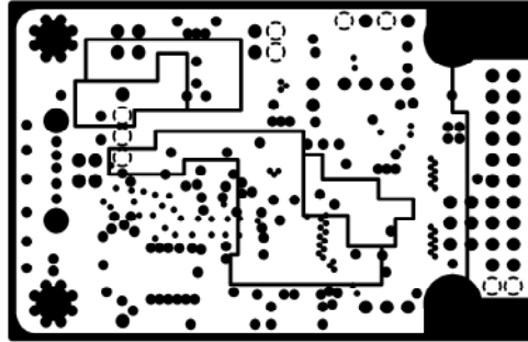
INTERNAL PLANE2
