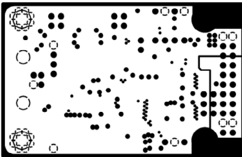
INTERNAL PLANE1
