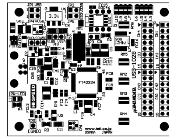
Component Side
