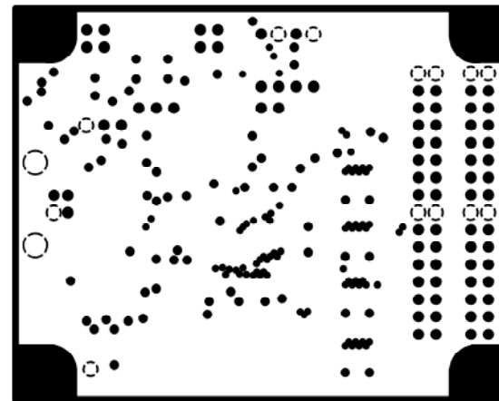
INTERNAL PLANE1
