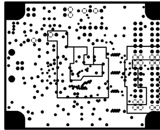
INTERNAL PLANE2
