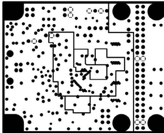
INTERNAL PLANE2
