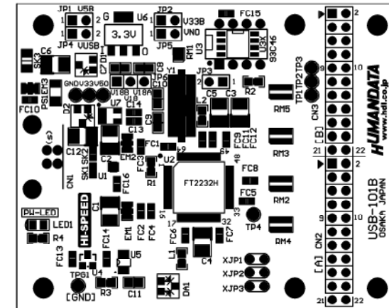
Component Side
