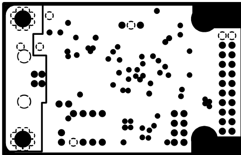
INTERNAL PLANE1
