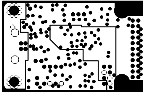
INTERNAL PLANE2
