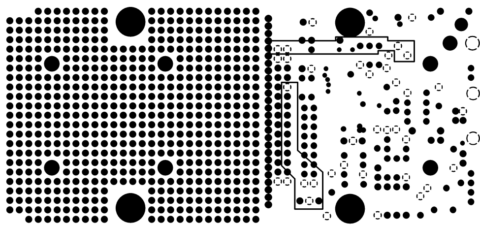
INTERNAL PLANE 1
