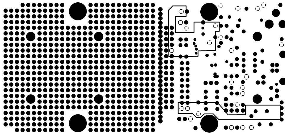
INTERNAL PLANE 2
