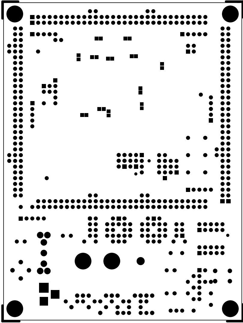
Bottom Solder Mask
