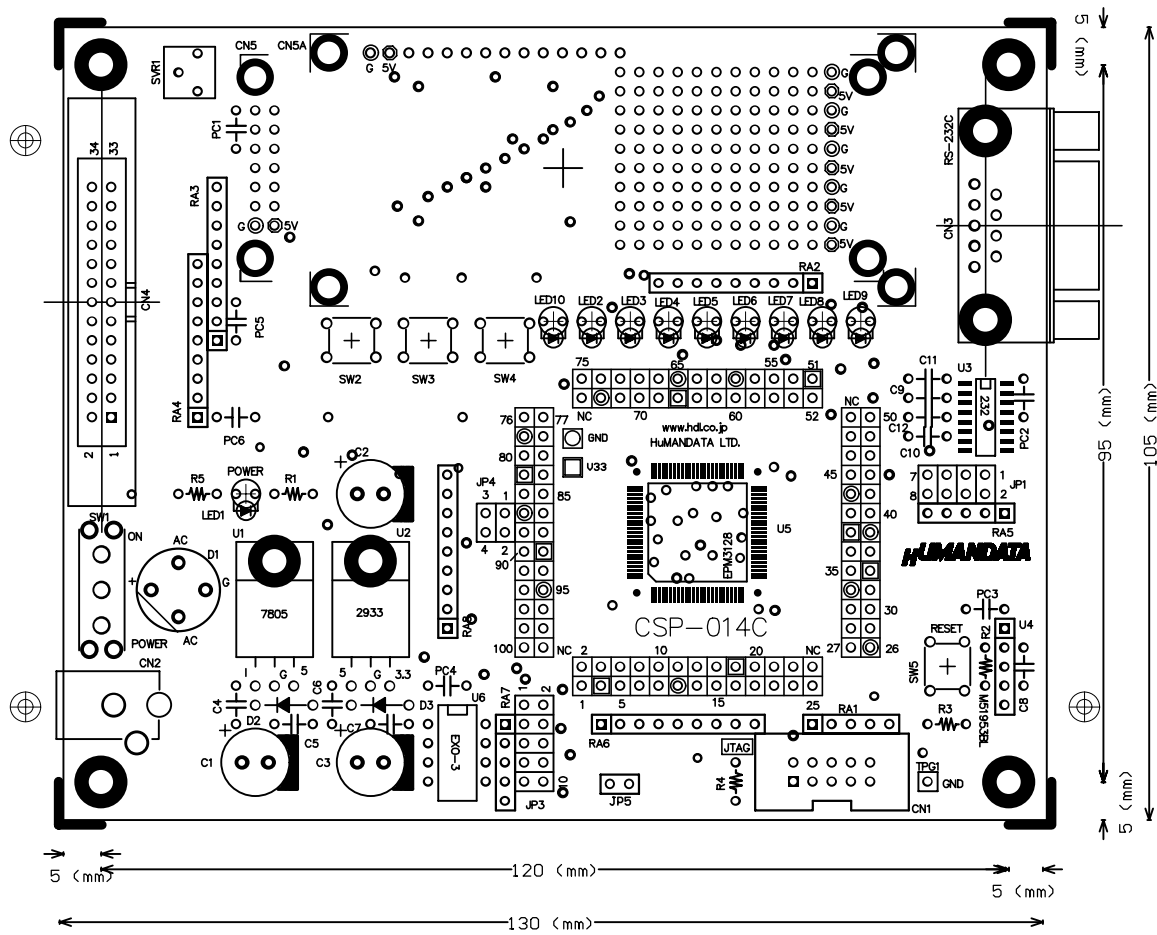
Top Overlay KJHC-KJI2
