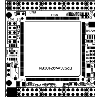
Component Side
