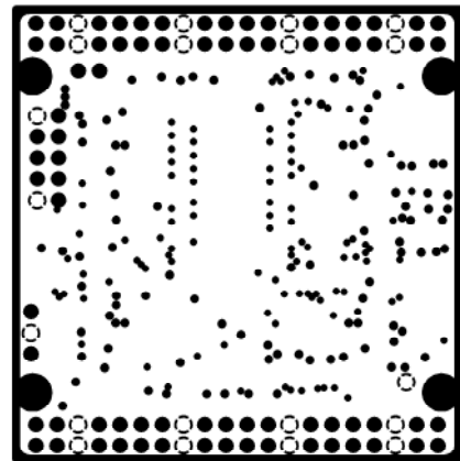
INTERNAL PLANE1
