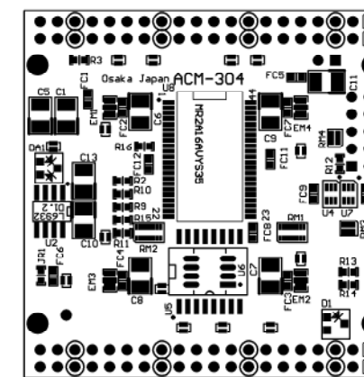
Solder Side
