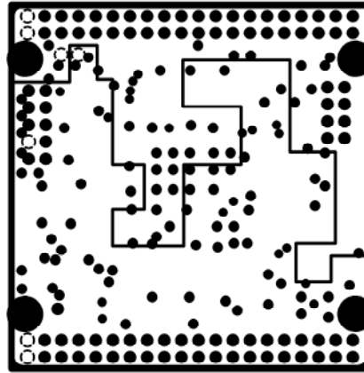
INTERNAL PLANE2
