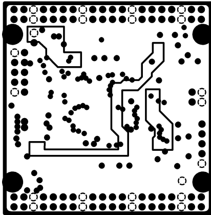
INTERNAL PLANE1
