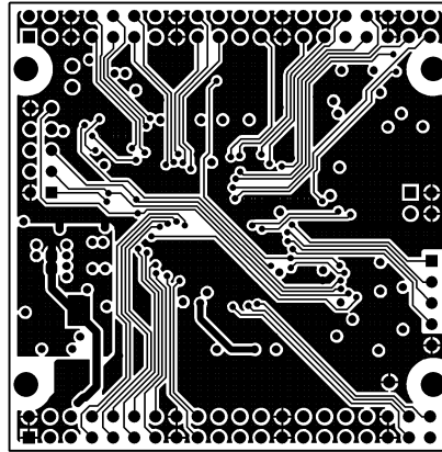
INTERNAL PLANE2
