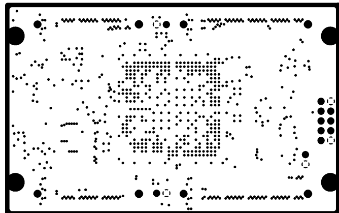
INTERNAL PLANE 1
