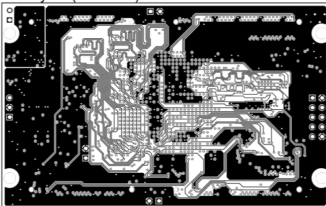
MidLayer2 (Scale 1:1)
