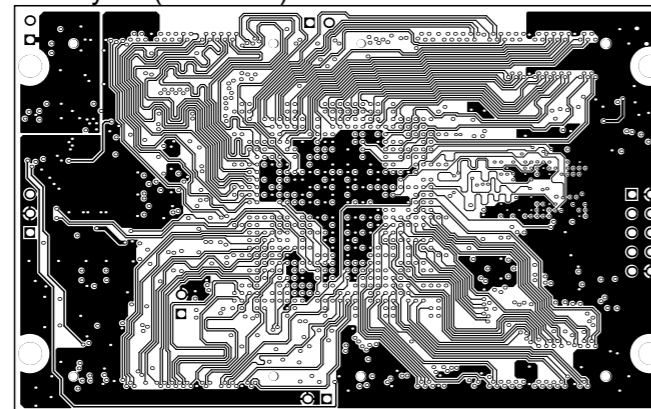
MidLayer1 (Scale 1:1)
