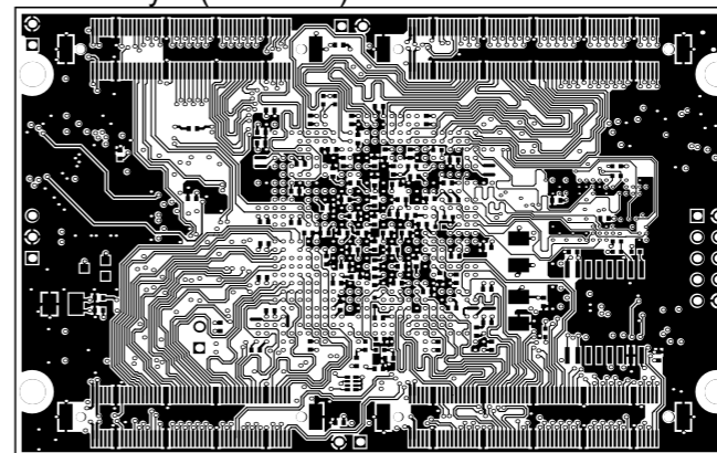
BottomLayer (Scale 1:1)
