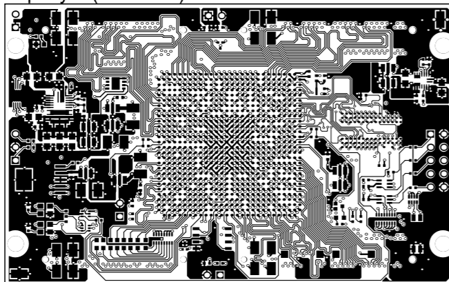
TopLayer (Scale 1:1)
