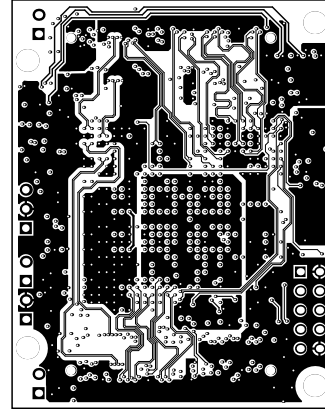
Signal Layer 3 (Scale 1:1)
