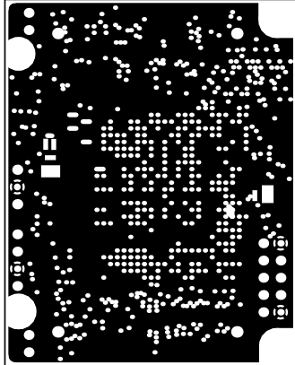
Internal Plane 1 (Scale 1:1)
