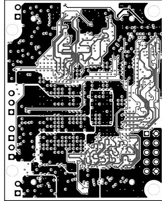
Signal Layer 1 (Scale 1:1)
