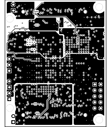
Signal Layer 4 (Scale 1:1)
